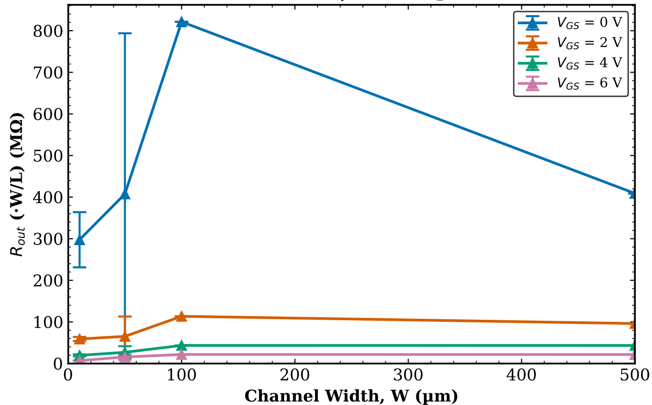
TFT1 Combined (Tr. 1 & 2) R_{out} vs W | L = 80\text{ }\mu\text{m}
